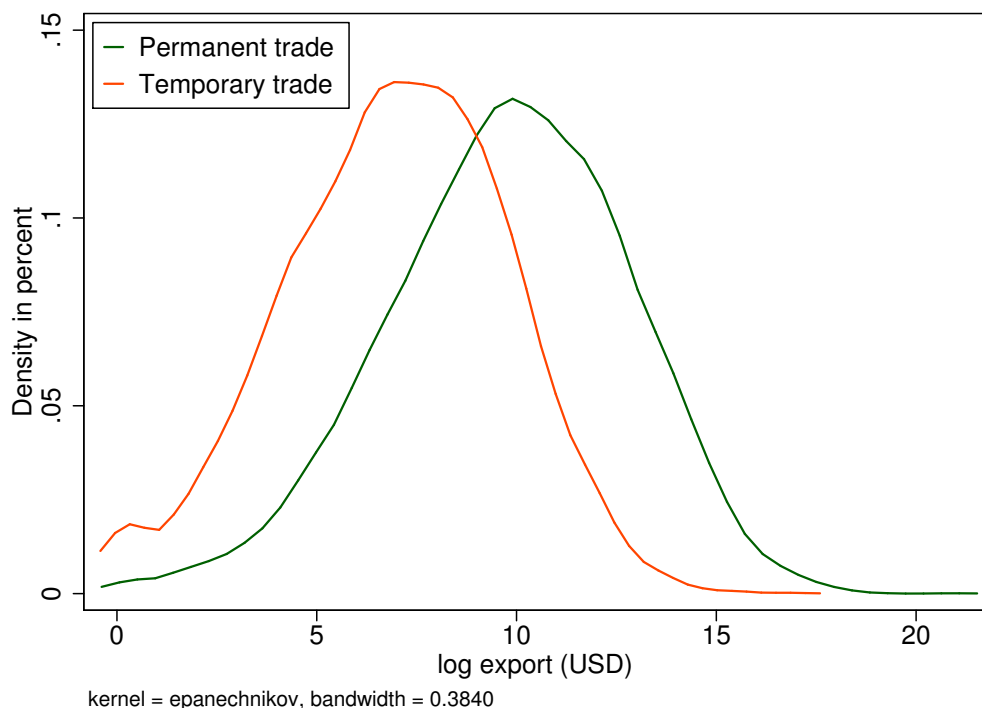
Fig. 4. Kernel densities of permanent and temporary trade
