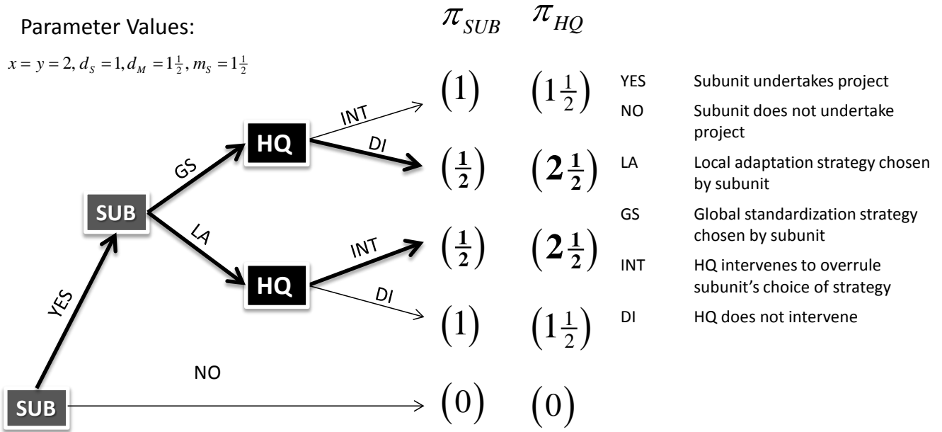
Figure 4: Necessary and beneficial intervention
