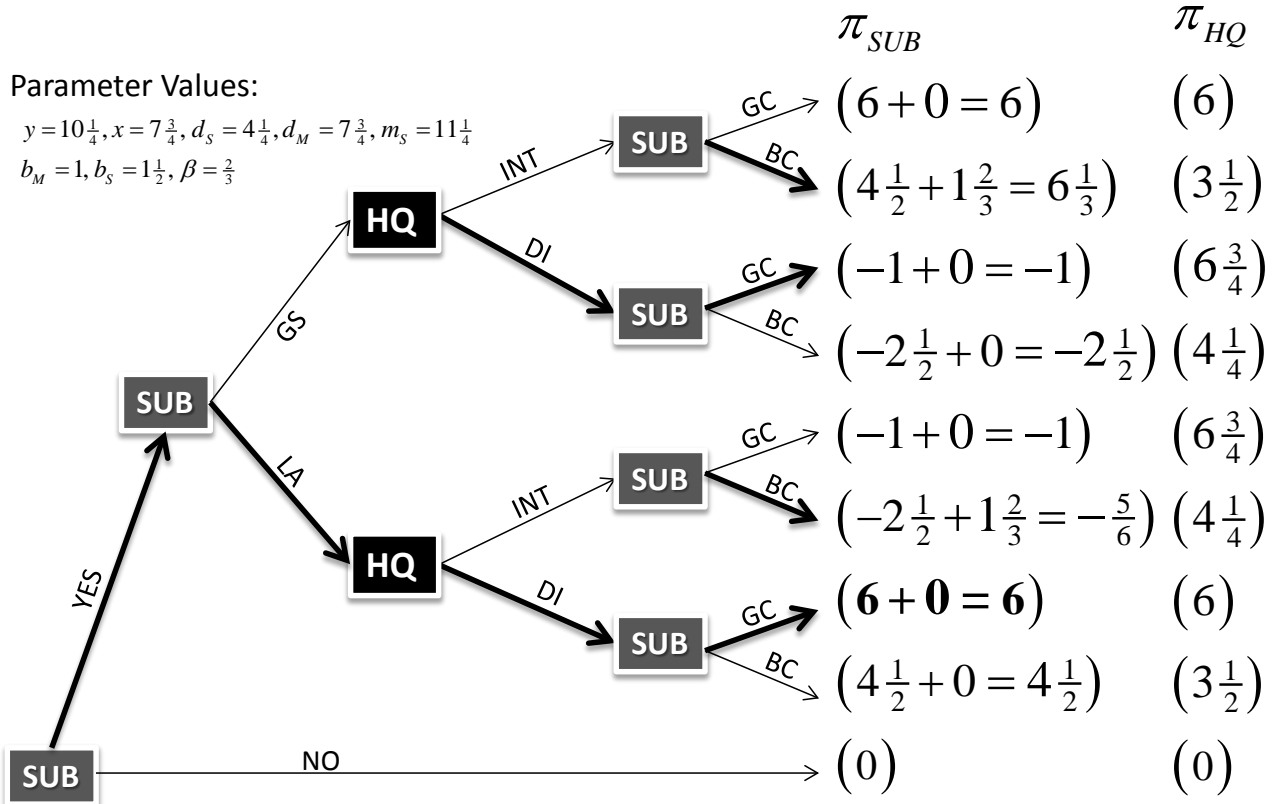
Figure 3: PJ and credible delegation
